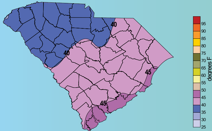
March Average Minimum Temperature (1971-2000)
