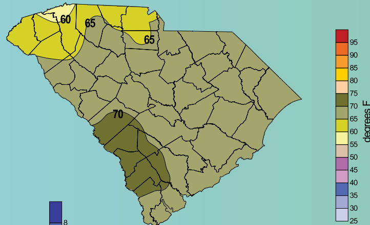
March Average Maximum Temperature (1971-2000)
