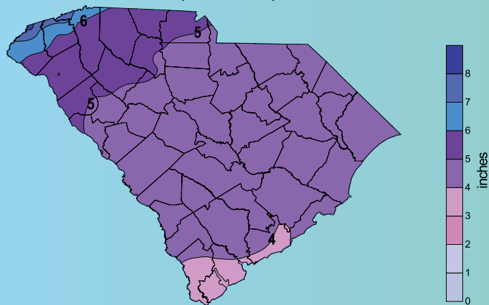
March Average Precipitation (1971-2000)
