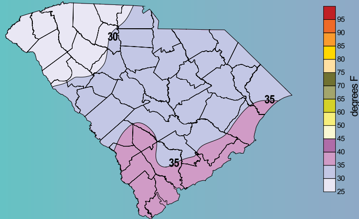
January Average Minimum Temperature (1971-2000)
