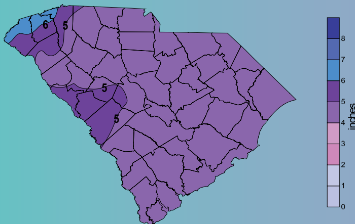
January Average Precipitation (1971-2000)
