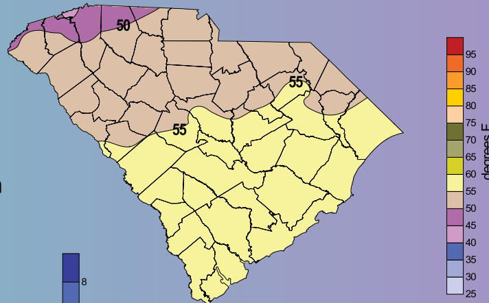
January Average Maximum Temperature (1971-2000)
