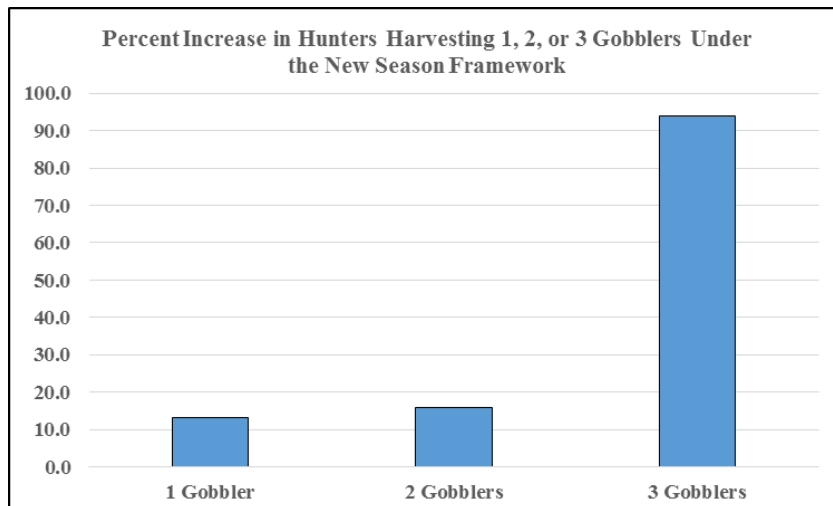
Figure 4. Percent increase in hunters harvesting 1, 2, or 3 gobblers under the new season framework in South Carolina. The percentage of hunters at each harvest level increased under the new season framework with the percentage of hunters who harvested 3 birds harvested increasing over 90 percent compared to the old season framework.
