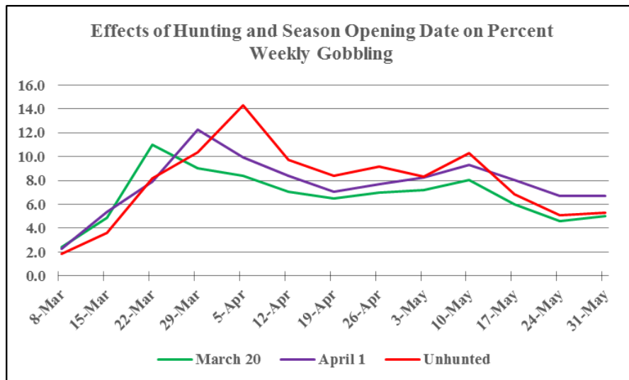
Figure 7. Effects of hunting and season opening date on percent weekly gobbling in South Carolina. Compared to the “natural” gobbling distribution documented on the unhunted study area the onset of hunting immediately and negatively affects gobbling. Data for the March 20 opening date was predicted based on the relationship between gobbling data collected on the unhunted study area compared to 2 areas where hunting began the Saturday before April 1 (youth turkey day).
