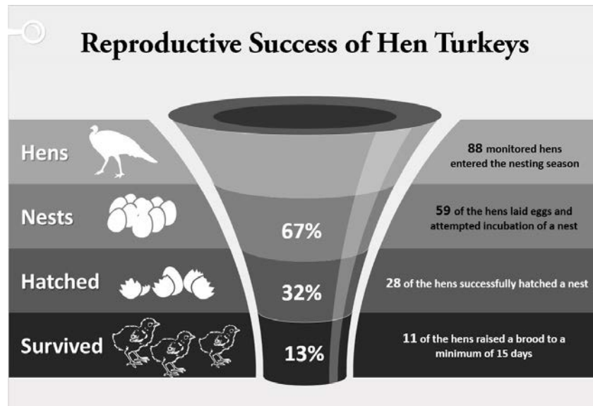
Figure 9. Nesting success for female wild turkeys on Webb WMA Complex in South Carolina 2015-2018.
