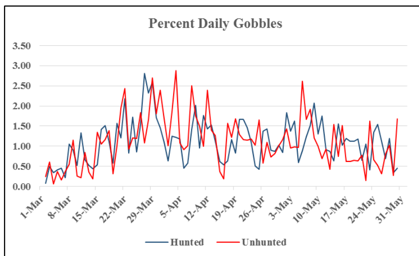
Figure 5. Percent of total gobbles by day for unhunted and hunted sites in South Carolina during 2015-2018. Total number of gobbles heard was 91,102. Note extreme variation in daily gobbling activity during the turkey reproductive and hunting seasons and decrease in gobbling activity on the hunted sites from early to mid-April.
