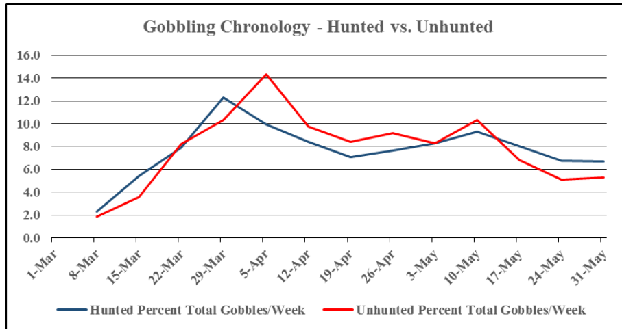
Figure 6. Comparison of the timing and distribution of gobbling between hunted and unhunted study areas in South Carolina. Gobbling is immediately and negatively affected by the onset of hunting through a combination of gobblers being killed and disturbance from hunters.
