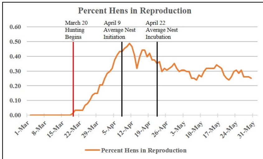
Figure 8. Percent of hen turkeys in reproduction in South Carolina 2015-2018. In reproduction refers to egg-laying, incubating, and brooding. The current March 20 season opening date is 20 days prior to the April 9 date of average nest initiation (egg-laying) and 33 days prior to the April 22 date of average nest incubation.
