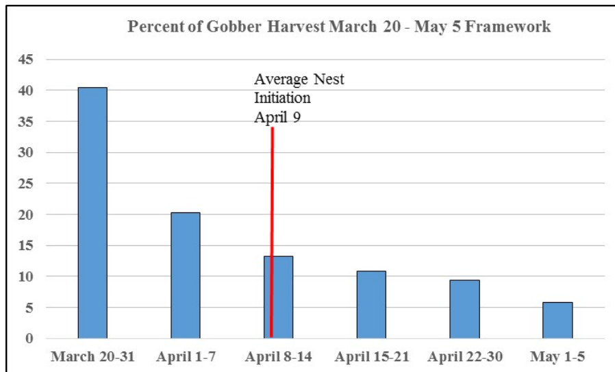
Figure 10. Percent gobbler harvest by week in South Carolina 2016-2018. Under the current March 20 opening date in South Carolina, approximately 60 percent of the annual gobbler harvest occurs prior to average date of nest initiation (egg-laying) by hens. These gobblers are immediately lost from a reproductive standpoint which could affect successful reproduction by hens.
