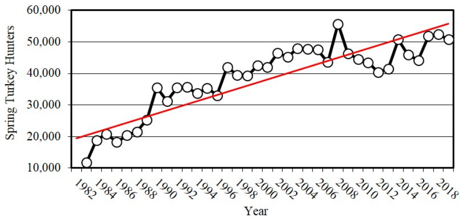
Figure 2. Number of spring turkey hunters in South Carolina 1982-2018 demonstrating increasing hunters over time ( R^2 = 0.75 ).
