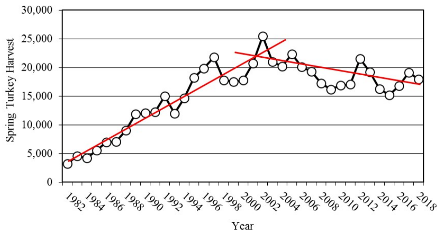
Figure 1. Spring wild turkey harvest in South Carolina 1982-2018. Harvest increased ( R^2 = 0.92 ) between 1982 and 2002 as a result of increasing turkey population during restoration efforts. Since 2002 harvest has generally decreased, although harvest has been up an average of 18 percent during the 3 years of the new season framework.
